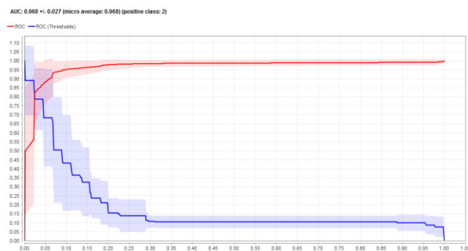
Gambar 14 Kurva ROC Algoritma C4.5 + PSO
