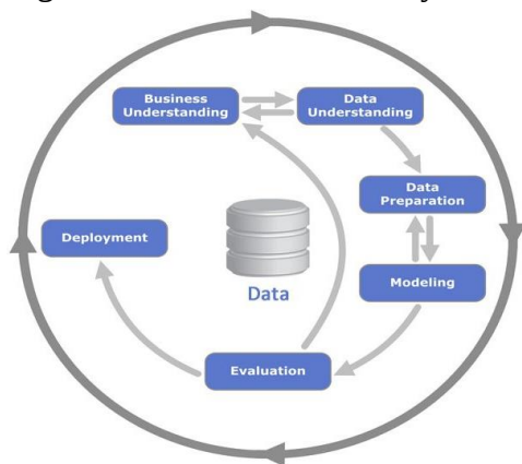
Gambar 1. CRISP-DM
